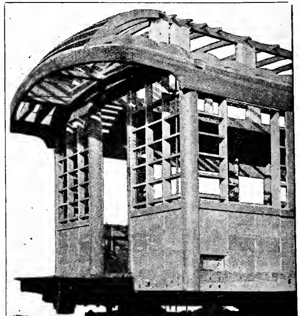
Fig. 535. Corner View, showing Hood, End and Side Framing.
